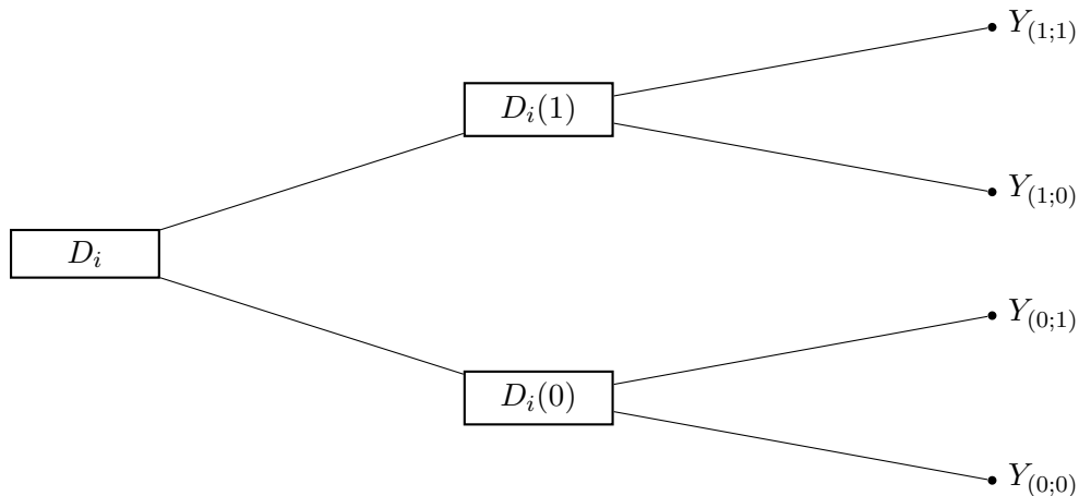
Figure 1: Decision Tree
